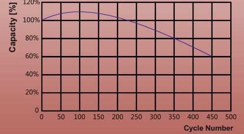
Cycle Life - Remaining Capacity Relationship [25°C]
