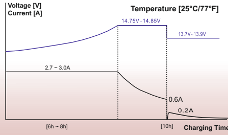
Charge Characteristics [25°C]
