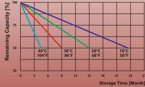
Time - Self Discharge Relationship
